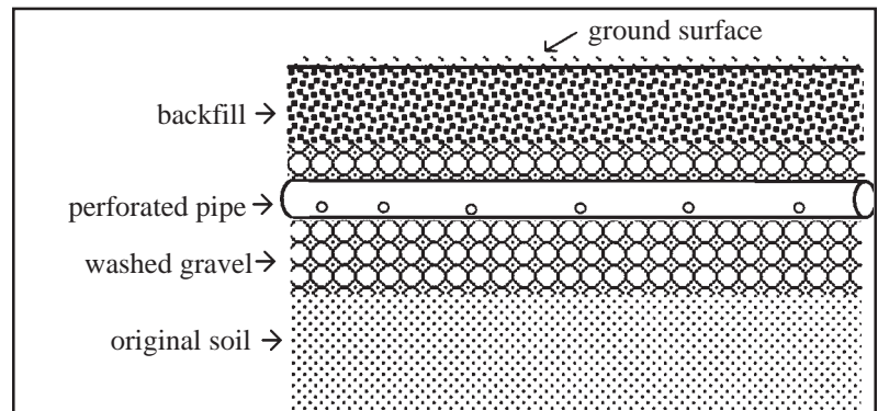
Figure 4 Septic Drainfield, Courtesy—Washington State University
