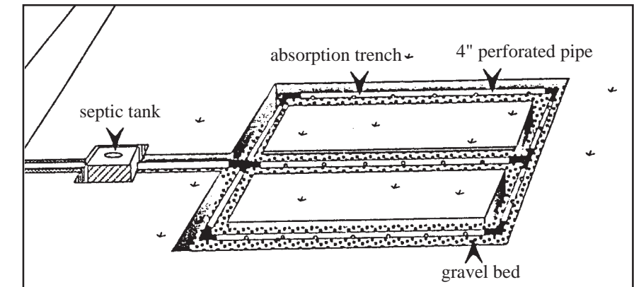
Figure 1: Septic System —Courtesy National Small Flows Clearinghouse
