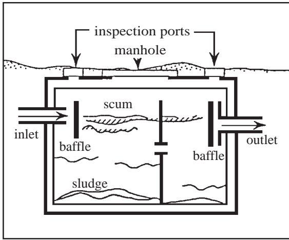
Figure 2: A Two-Compartment Septic Tank— Courtesy National Small Flows Clearinghouse
